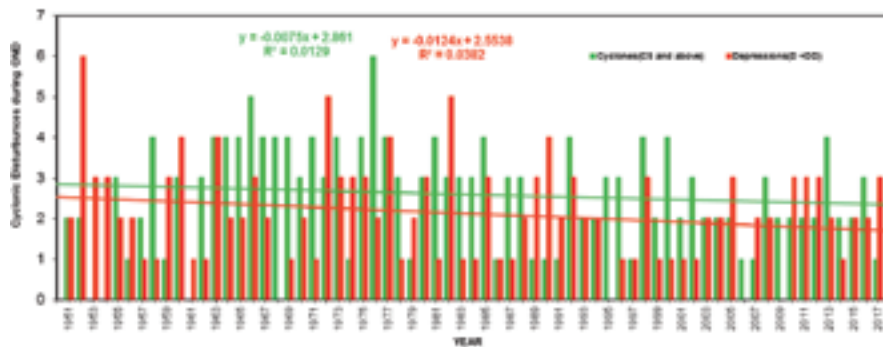
Figure 1.8 (a) and (b): Frequency of depressions and cyclonic storms formed over the northern Indian Ocean (1951-2017). Source: IMD
